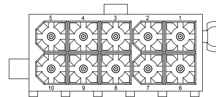
2X5PIN
