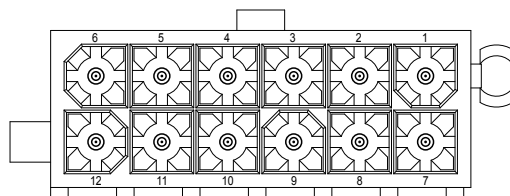
2X6PIN
