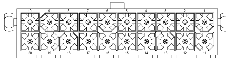
2X10PIN
