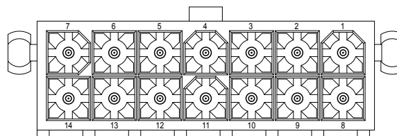
2X7PIN
