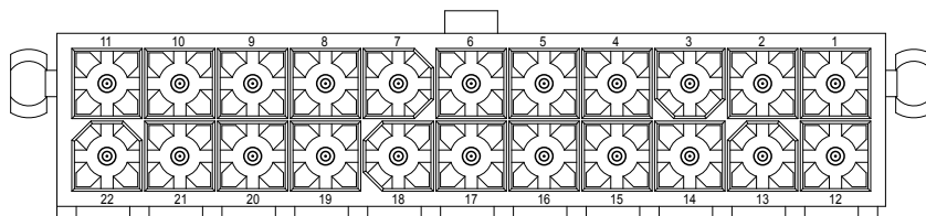
2X11P
