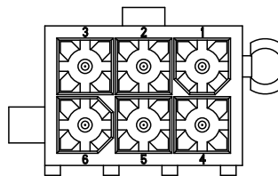
2X3PIN
