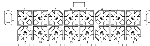
2X8PIN
