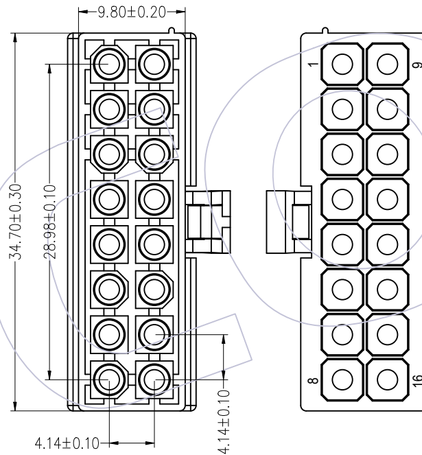
2X8PIN
