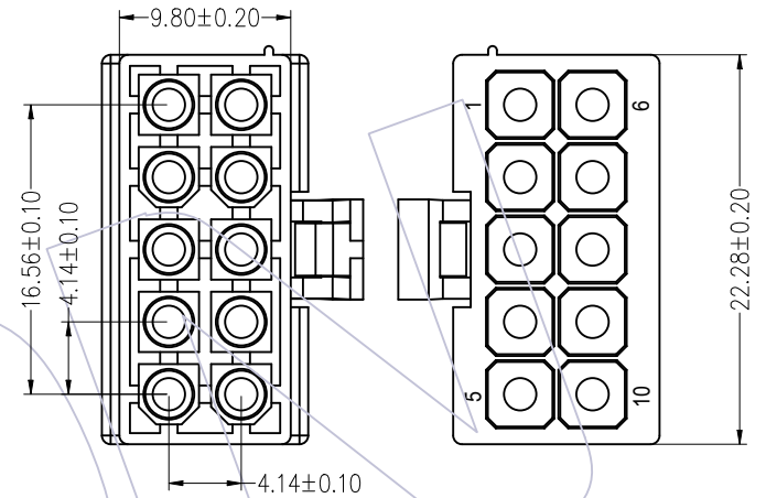
2X5PIN
