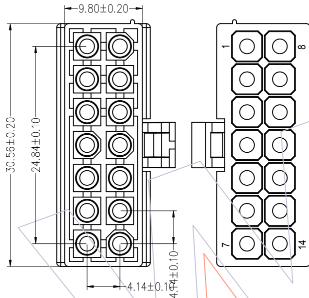
2X7PIN
